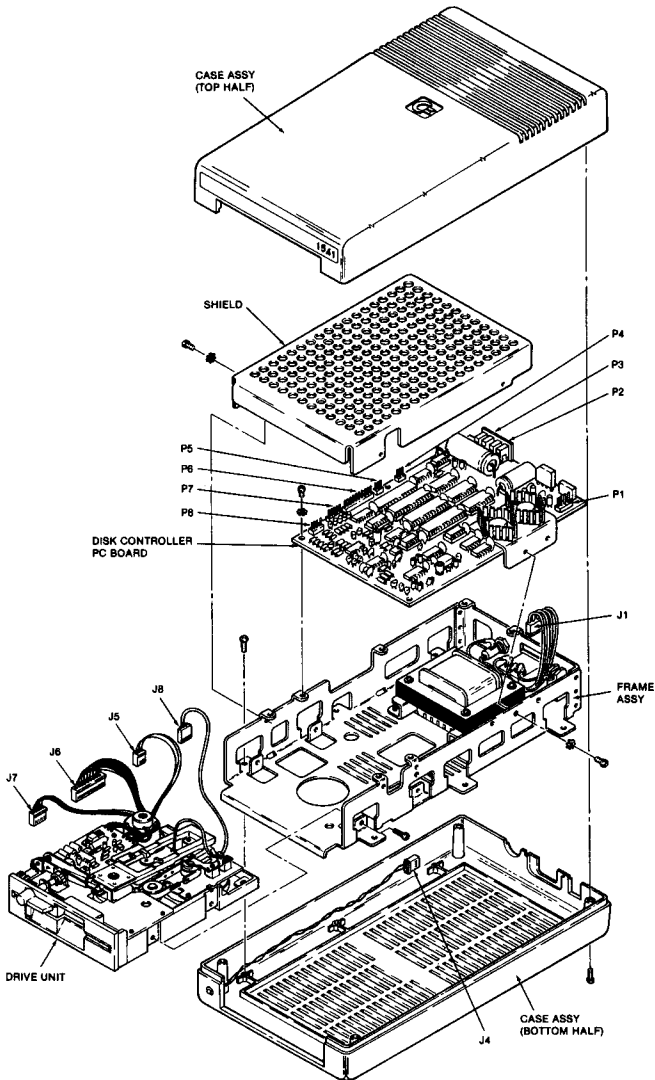
Fig. A-15. Subassembly identification, Model 1542.
